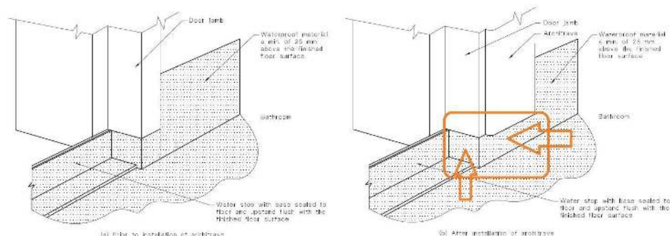
FIGURE 3.3 TYPICAL BATHROOM DOOR DETAIL FOR WHOLE BATHROOM WATERPROOFING
