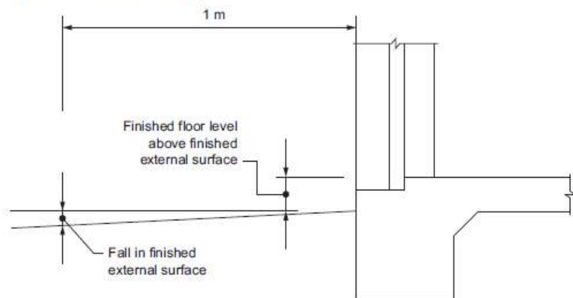
Figure 3.3.3a: Site surface drainage
