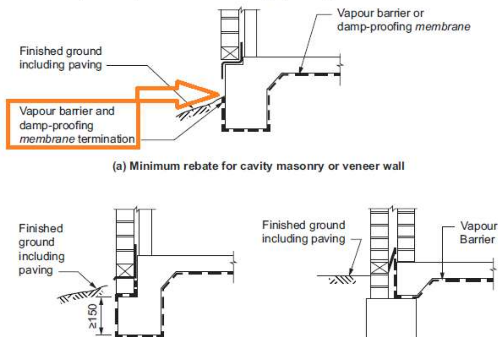
Figure 4.2.8: Acceptable vapour barrier and damp-proofing membrane location
